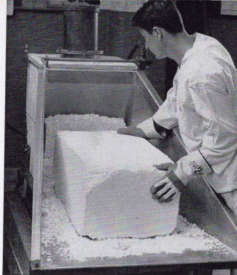
Bale of cellulose acetate being broken up and dumped into a solution containing solvents.
